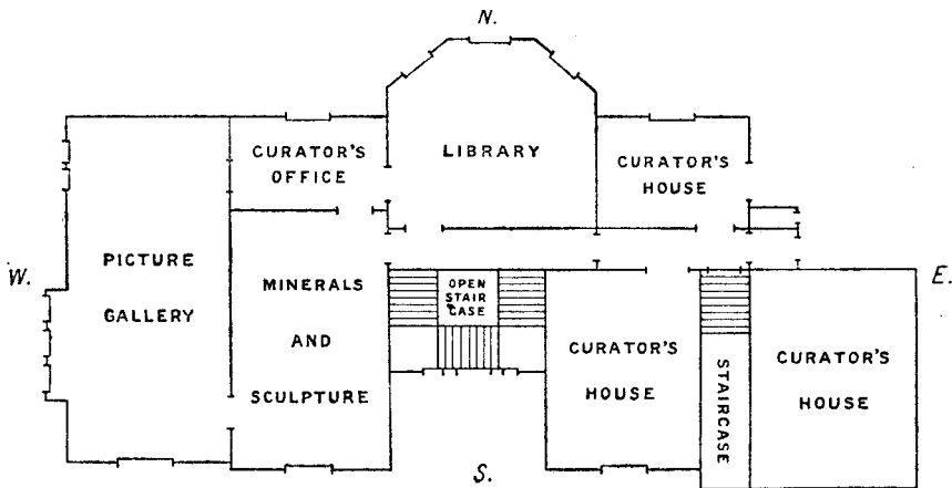
FIRST FLOOR
